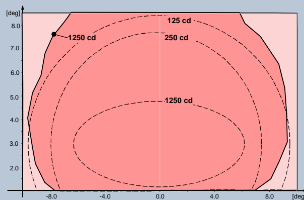
Fig. 2 ICAO A2-8 – Red
