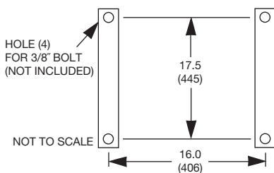
Mounting Channel Bolt Hole Pattern
